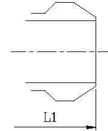
Buttwelding Ends
